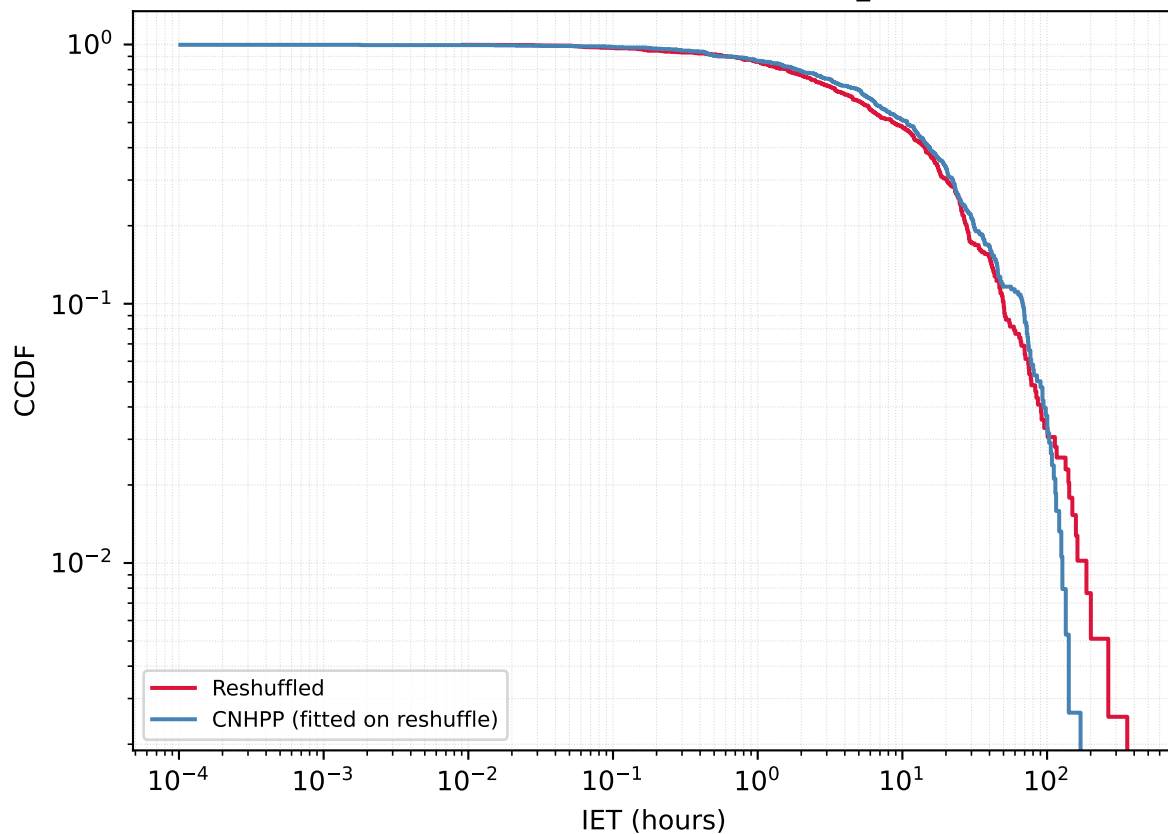
User 412633448 - Reshuffled vs CNHPP A_{\text{fit}}=0.1304
